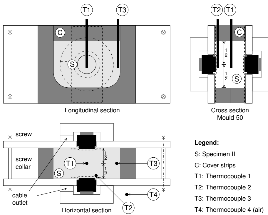
Figure 4: Thermocouple placement schema. Locations inside and outside of mould M2.
