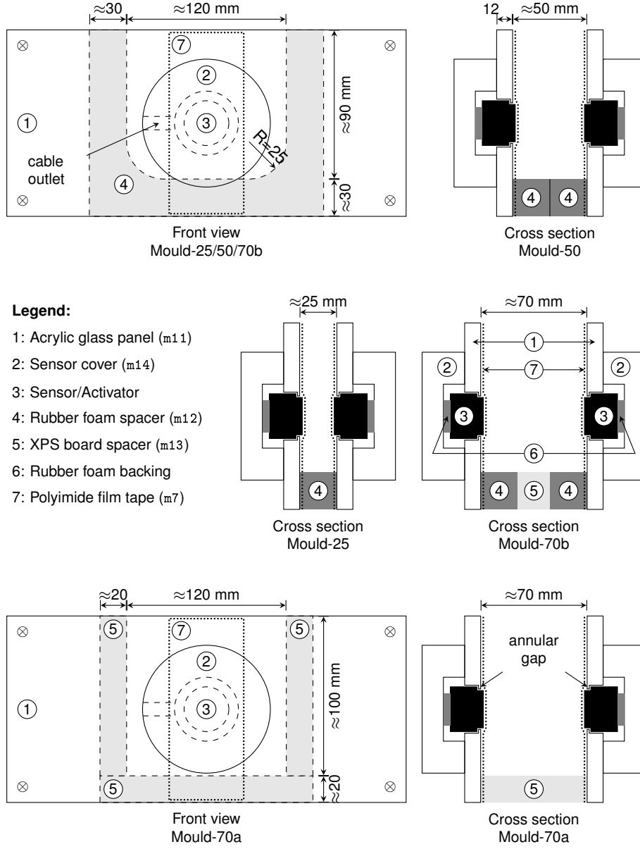
Figure 3: Schematic view of the ultrasound testing device' mould configuration. Note: mould M1 and mould M2 shown in Figure 2, p. 11 are, except the built-in ultrasonic contact probes, identically constructed. With respect to the ultrasonic measuring distance D , one of the four mould variants (Mould-25, Mould-50, Mould-70a, Mould-70b) was chosen. The material ID's (e.g. m11) mentioned in the legend refer to the materials listed in Table 6, p. 16.
