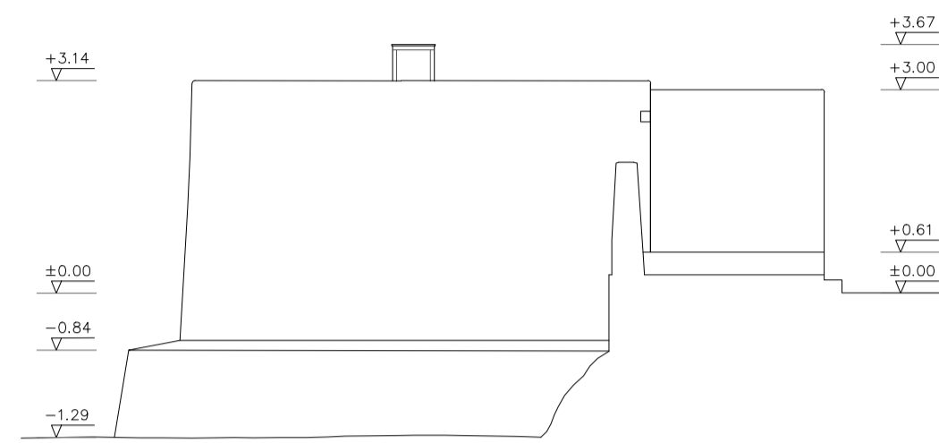
South elevation
