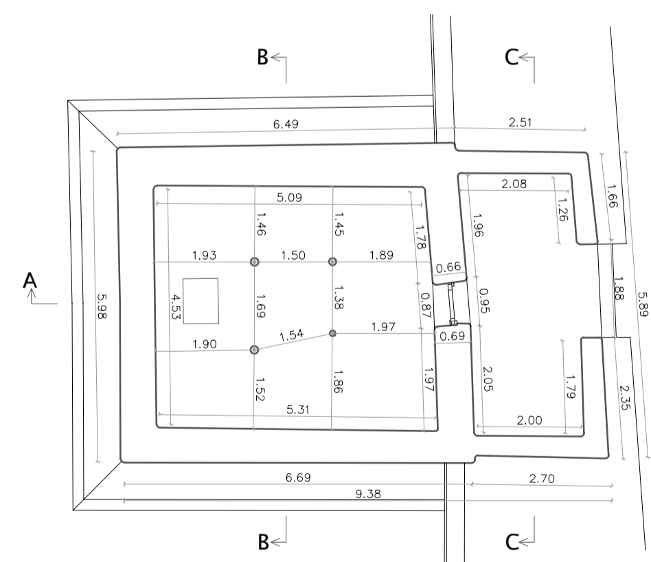
Floor plan
