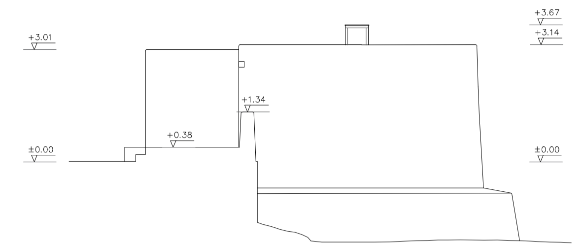
North elevation
