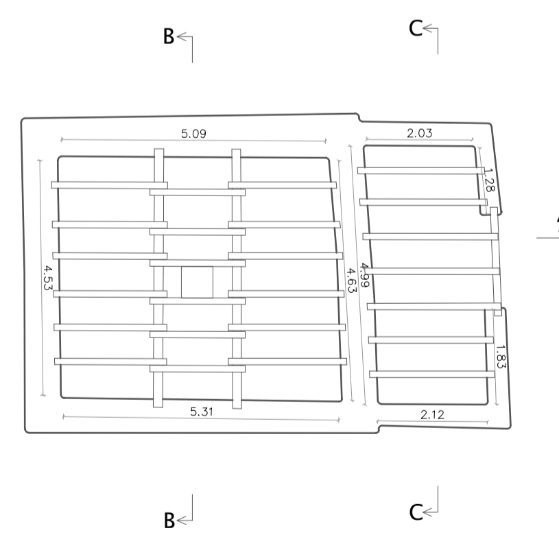
Ceiling plan
